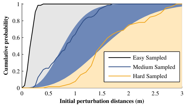
Figure 9 Cumulative probability as function of translation error for each of the perturbation set. The lines are based on the actual 64 samples; the filled backgrounds correspond to the theoretical curves. The easy sampled and theoretical curves overlay due to scaling.
